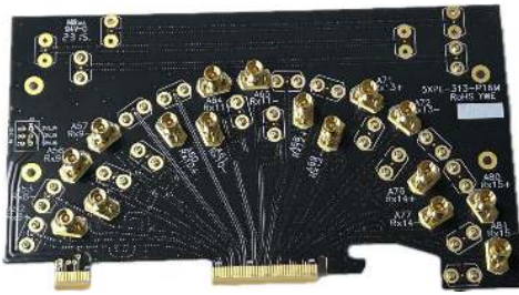
TF20-A-HTFD U4 Key A 20F fixture
