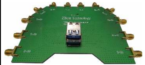
5R01T03 U3 TRL calibration fixture
