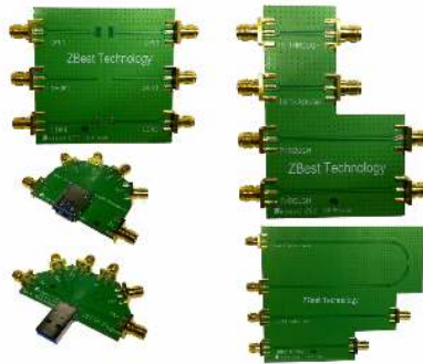
5R01T01 U3 open,short,Load calibration 5R01T02 U3 1X,2X calibration fixture 5R01T03 U3 TRL calibration fixture 5R09T01 U3 Female fixture
